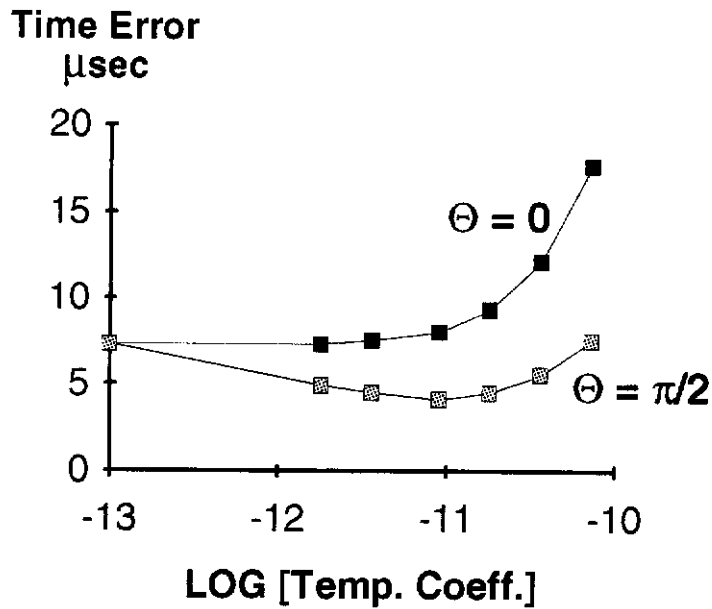
Figure 6: Satellite time error after 24 hours of free-running operation. Temperature coefficients for the satellite clock are per degree Celsius. The two curves labeled \theta = 0 and \theta = \pi/2 correspond to different phase relationships between the satellite's diurnal temperature cycle and the MCE's satellite correction cycle.
